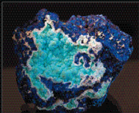
Chalcocite and Azurite - Bisbee, Arizona, USA
