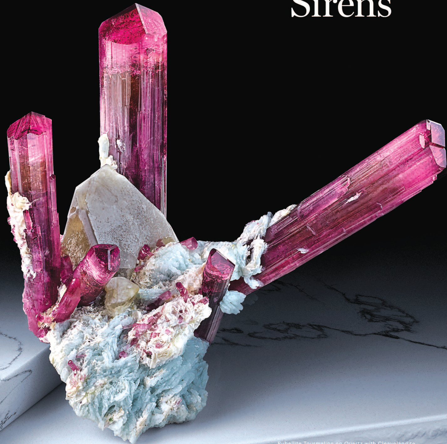
Rubellite Tourmaline on Quartz with Cleavelandite Malkhan Pegmatite Field, Krasnyi Chikoy, Zabaykalsky Krai, Russia 19 cm tall x 23 cm wide
