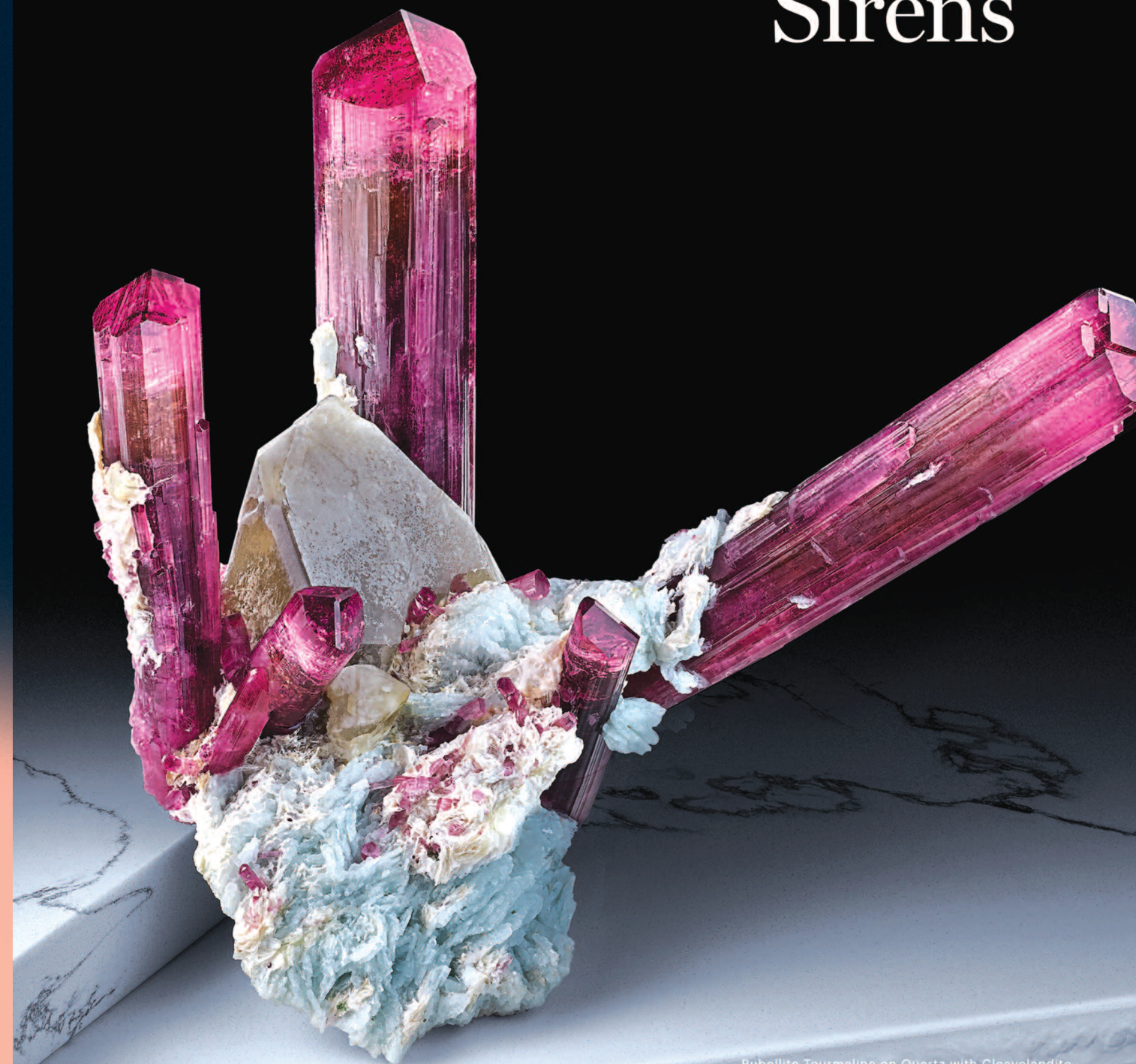
Rubellite Tourmaline on Quartz with Cleavelandite Malkhan Pegmatite Field, Krasnyi Chikoy, Zabaykalsky Krai, Russia 19 cm tall x 23 cm wide
