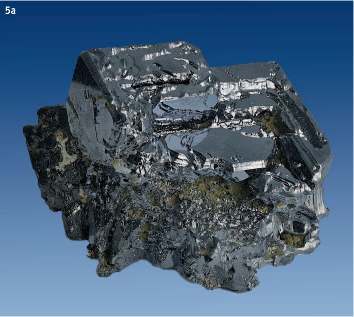
5a. Galena . 3 x 3 cm. Vtoroy Sovetsky mine, Dalnegorsk, Primorsky Krai, Russia. Specimen: Victor V. Ponomarenko.
