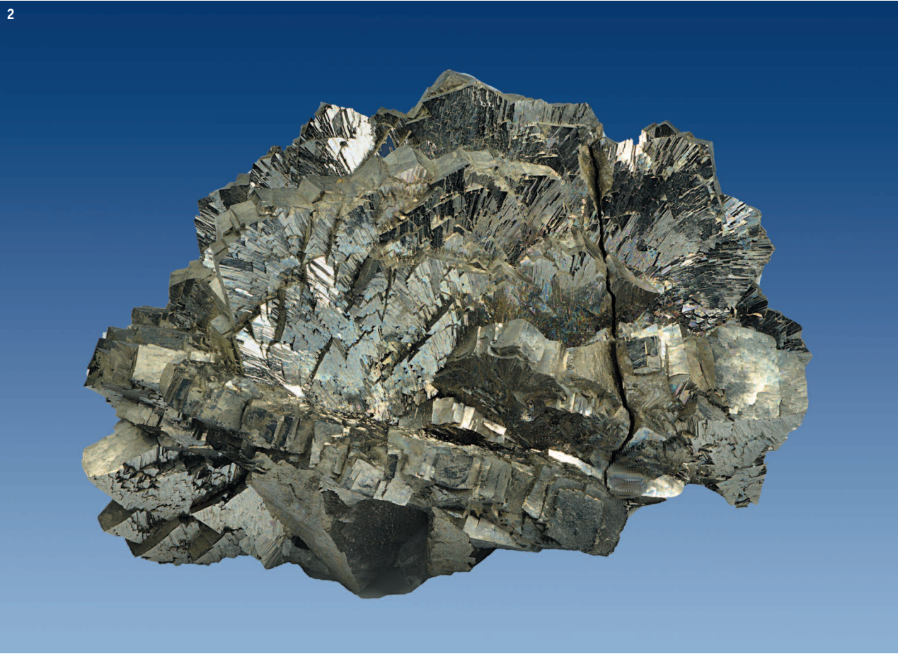
2. Arsenopyrite . 12 x 9 cm. Karalveem mine, near Bilibino, Chukotka Autonomous Okrug, Russia. Specimen: Victor V. Ponomarenko.
