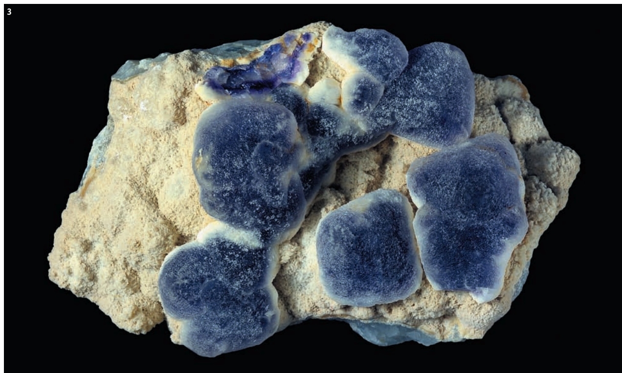
Figure 3. Fluorite. 13 x 18 cm. Khuraiskoe Deposit, Buryatia, Russia. "Russian Minerals" company specimen.
