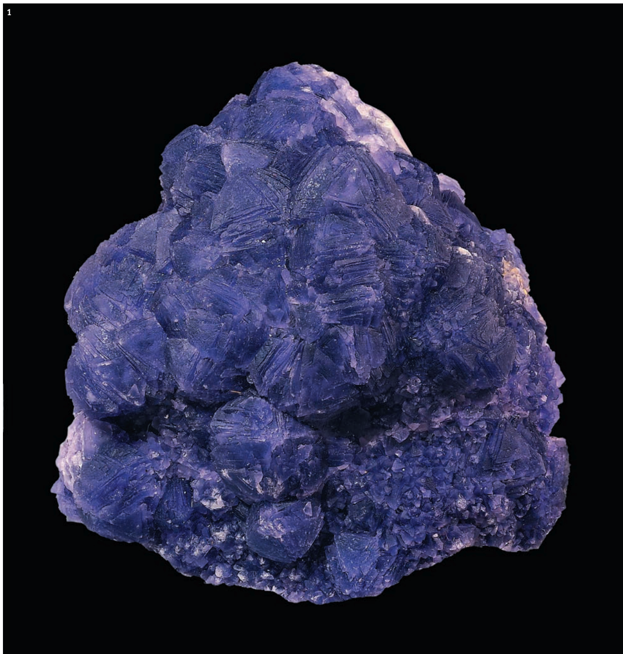
Figure 1. Fluorite. 24.5 x 27 cm. Khuraiskoe Deposit, Buryatia, Russia. D.I. Cherepanov specimen.
