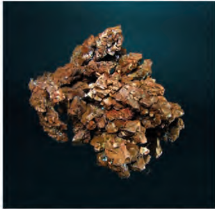
NEW FIND: CRYSTALLIZED COPPER 4.5 cm Poteryaevskoe deposit, Rubtsovsk, Altai, Russia Photo by Claudia Watson
